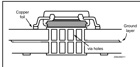
Figure 17: Mounting on epoxy FR4 using via holes for heat transfer of ground layer
