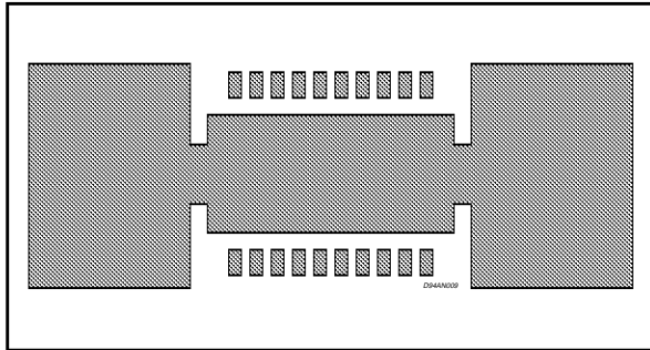
Figure 15: Footprint with dissipating element
