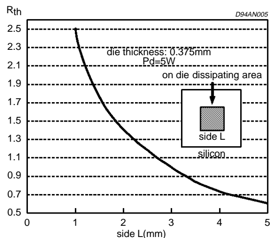
Figure 10: Thermal resistance junction-case vs. dissipating area of PowerSO-20
