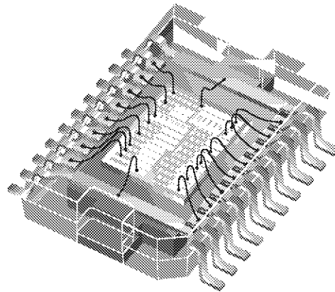
PowerSO-20™ – Jedec Registration MO-166
